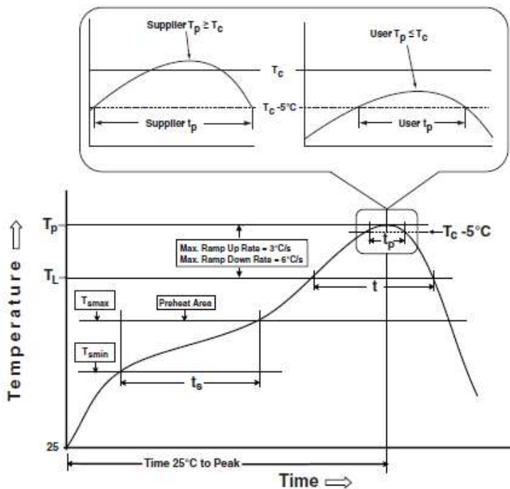
Fig.1 IR Soldering Reflow
